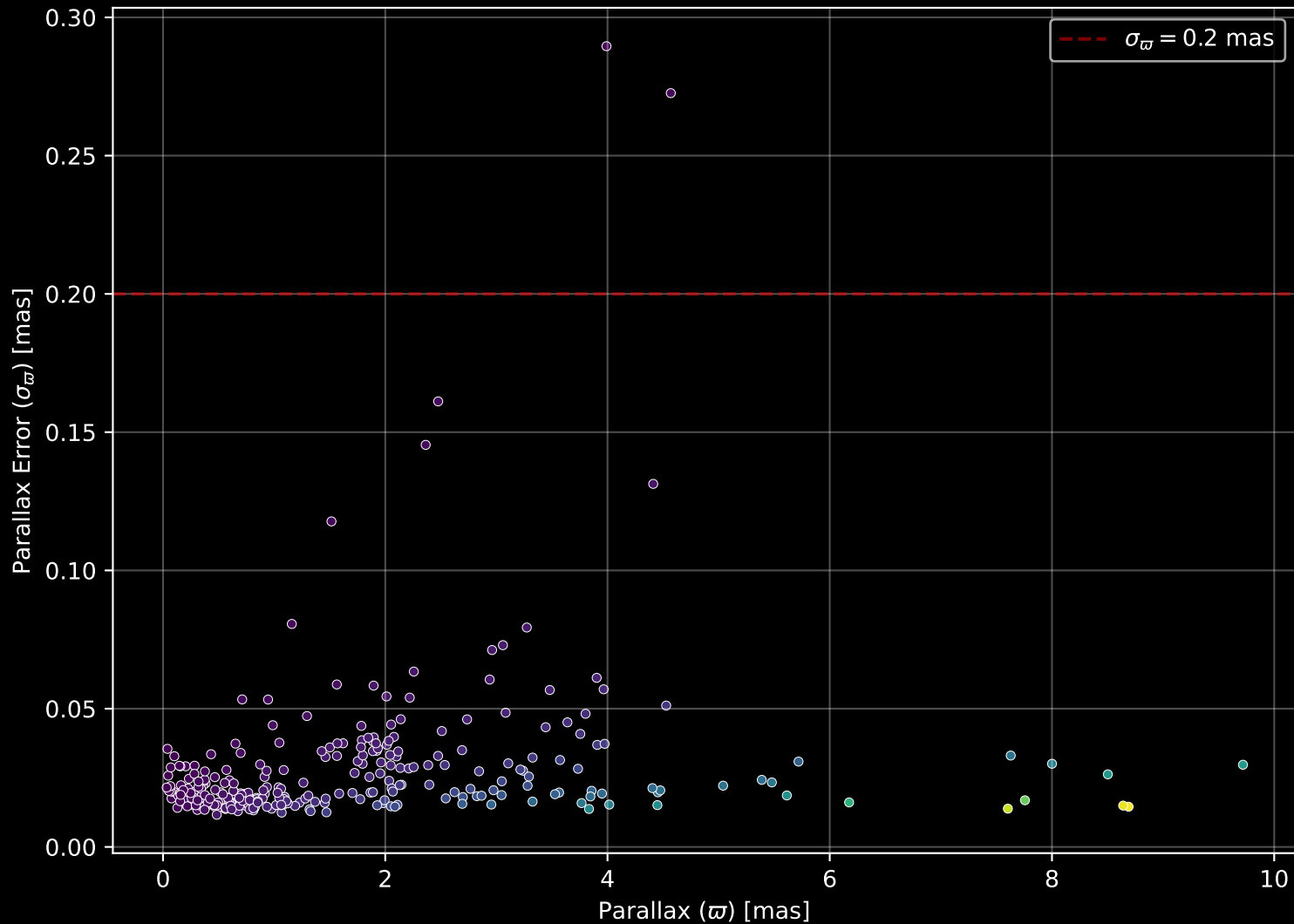
APOGEE DR17 Field: [186+31_btx] Parallax Quality (n= 304)
