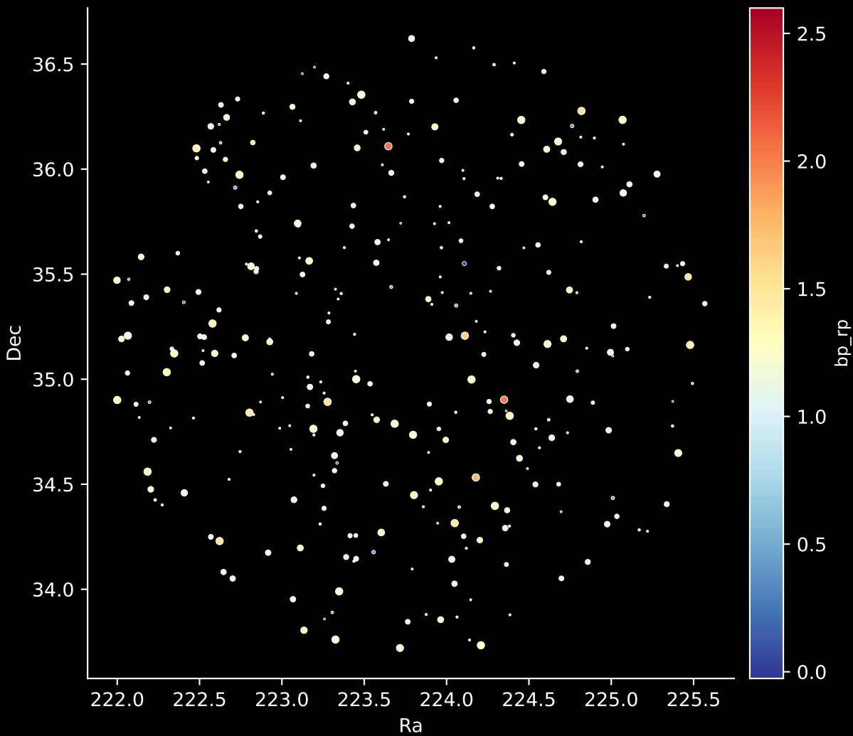
APOGEE DR17 Field: [186+31_btx] Stars: 304
