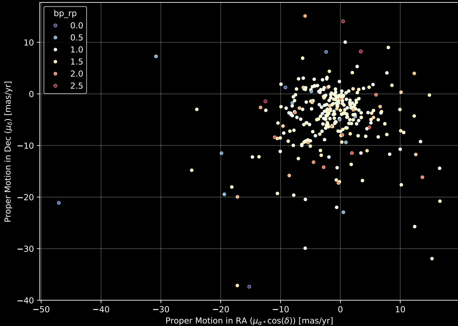
APOGEE DR17 Field: [186+31_btx] Proper Motion Diagram (n= 304)
