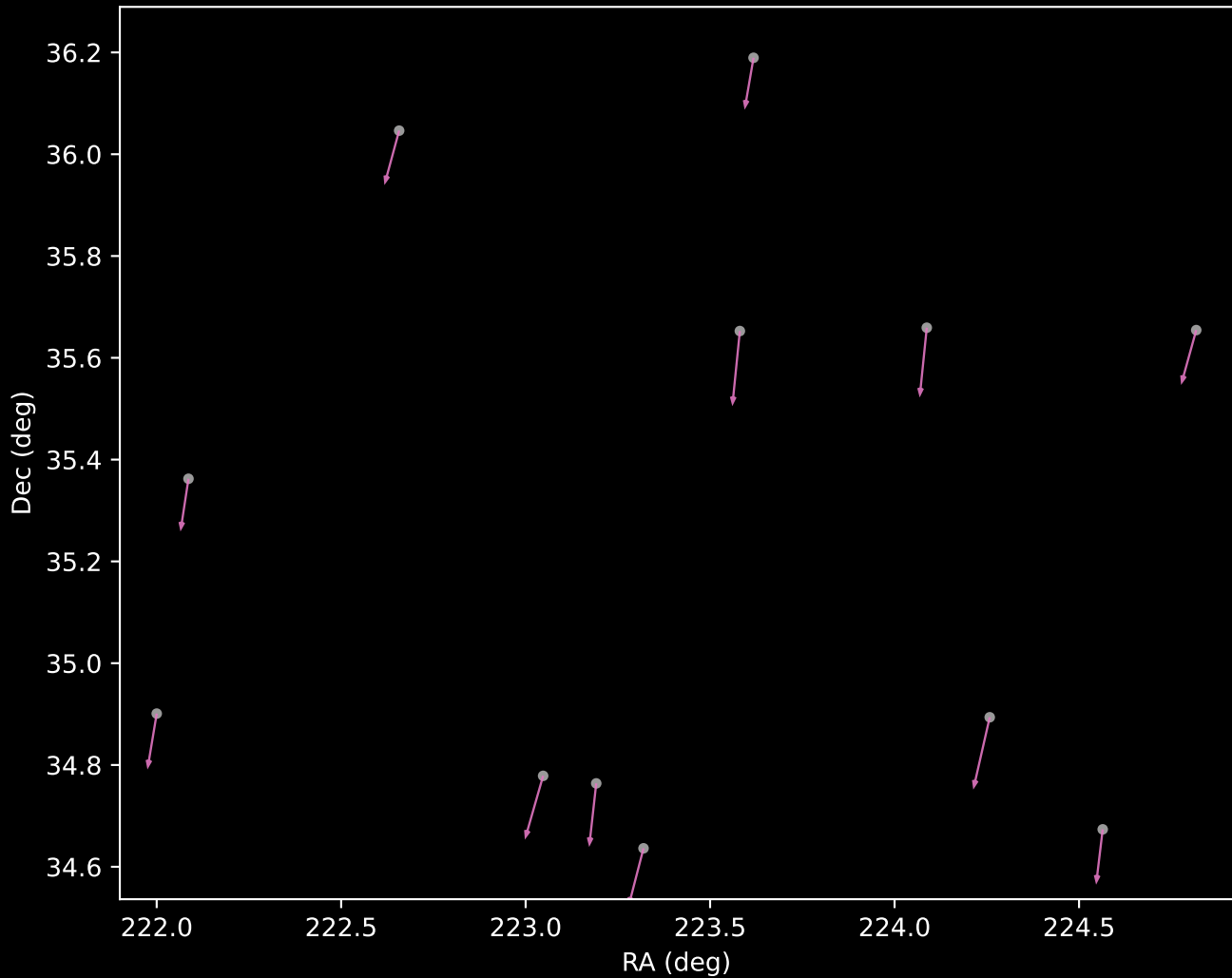
APOGEE DR17 Cluster 12 Proper Motion Vectors (n=12)
