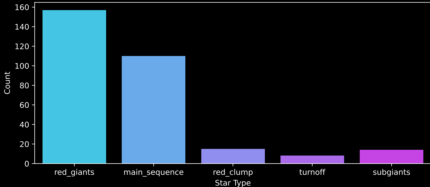
APOGEE DR17 Field: [186+31_btx] Count plot of Star Type
