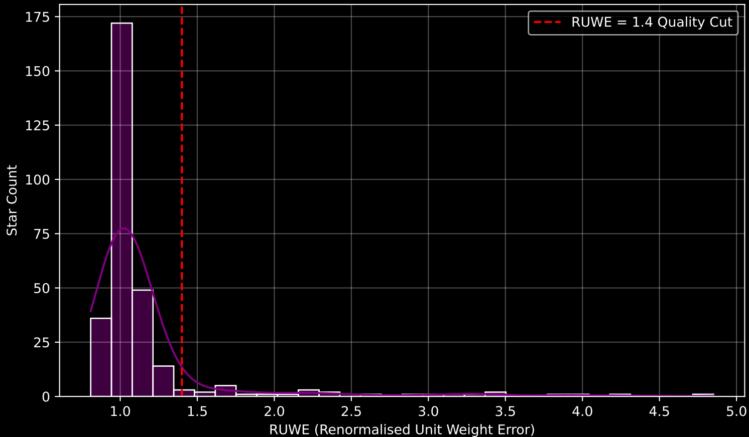
GAPOGEE DR17 Field [186+31_btx] RUWE Distribution (n= 300)
