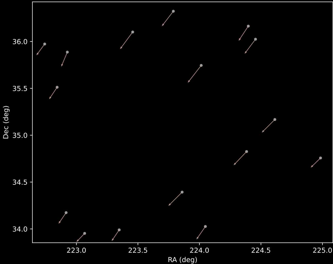
APOGEE DR17 Cluster 11 Proper Motion Vectors (n=16)
