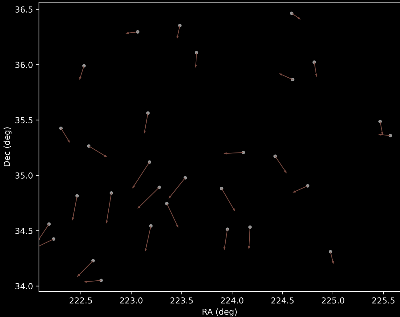
APOGEE DR17 Cluster 10 Proper Motion Vectors (n=30)
