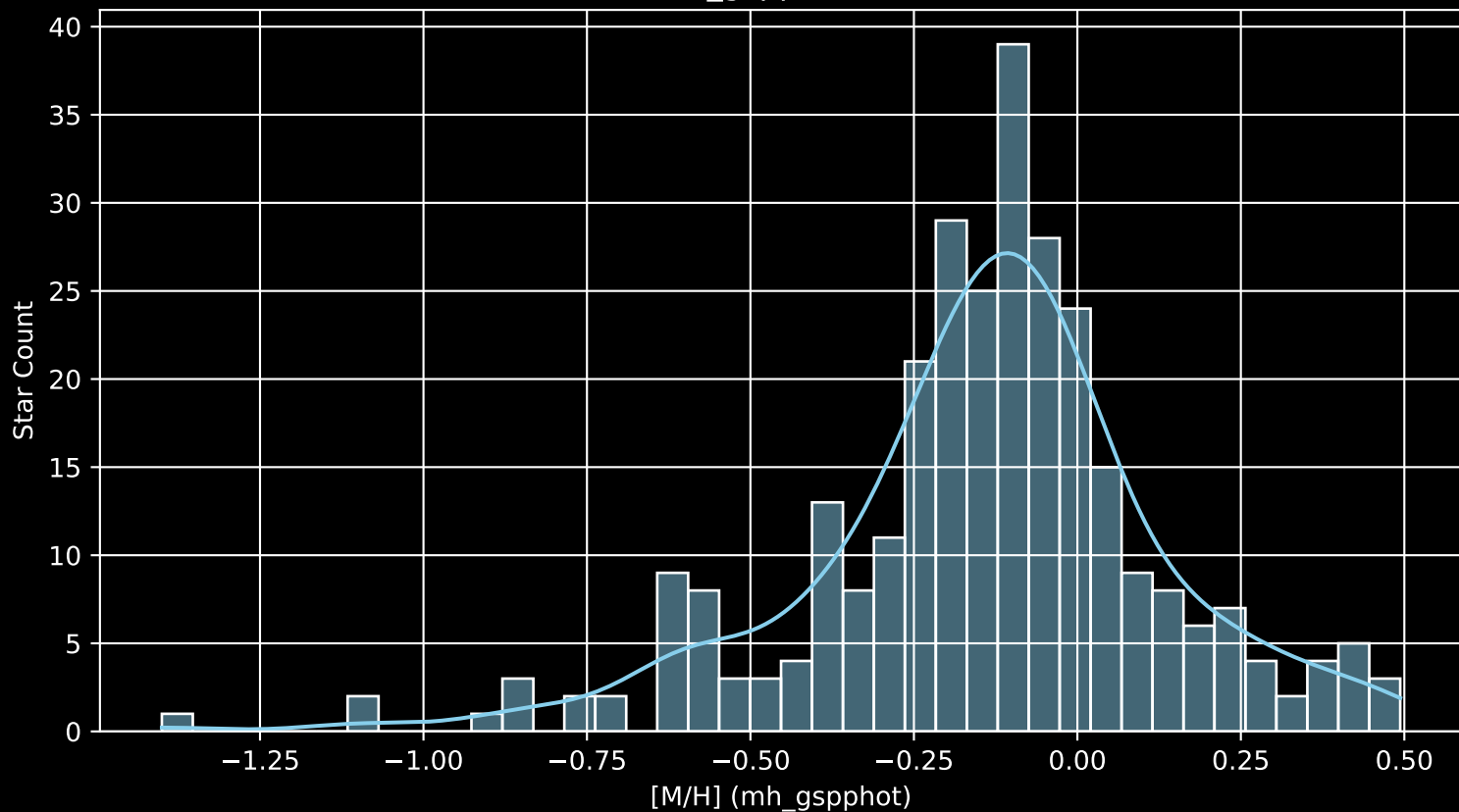
APOGEE DR17 Field: [186+31_btx [M/H] (mh_gspphot) (n= 299)
